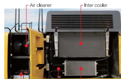
Battery Fuel cooler Radiator & Oil cooler
